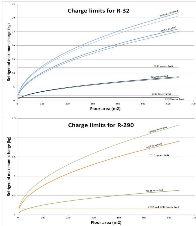
Figures 1a and 1b Charge limits for human comfort according to EN 378 Part 1 Annex C.2
