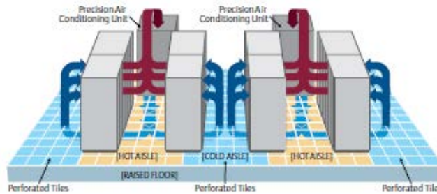
Figure A-8: Computer room air conditioner
