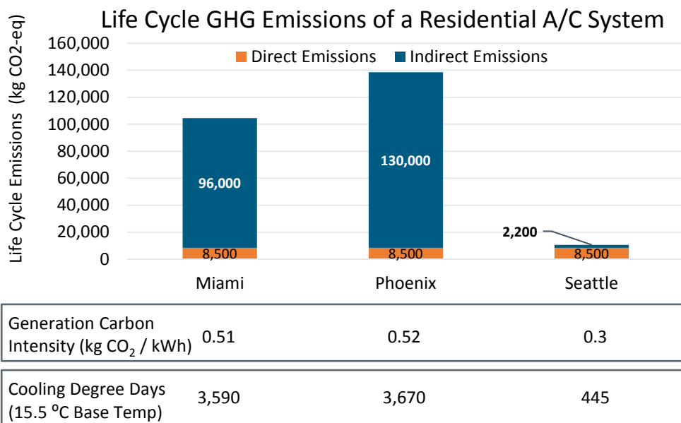
Figure 3-3: Life cycle GHG emissions of residential air-conditioning systems 55
