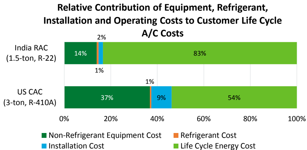
Figure 6-2: Residential life cycle A/C cost breakdown examples 136
